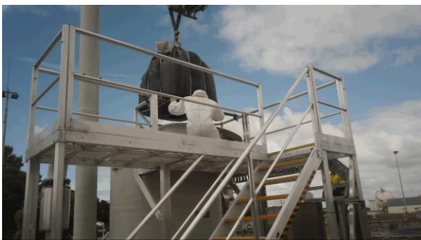
Loading the carbon filter medium
